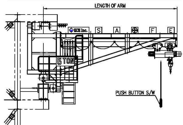
4. Pillar-Mounted Slewing Jib Crane(B)
