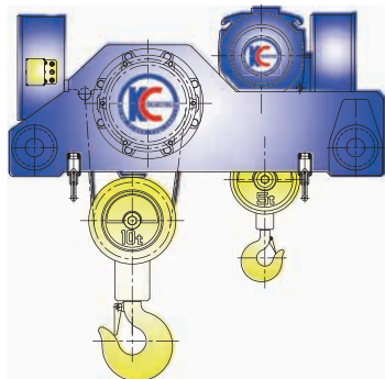
Main & Aux Type
