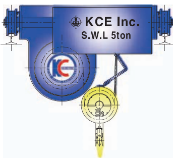
Double Low Head Type
